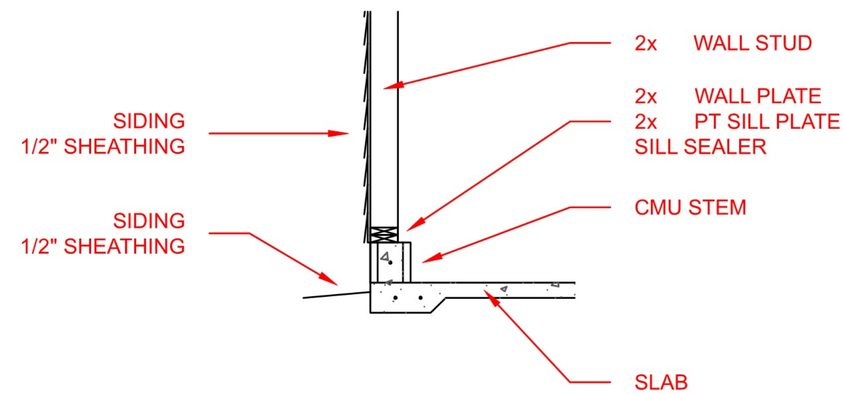
MONOLITHIC SLAB w/ STEM
