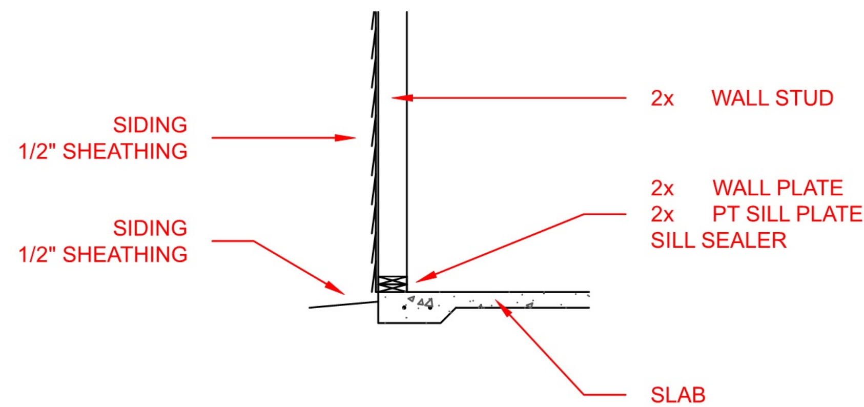
MONOLITHIC SLAB
