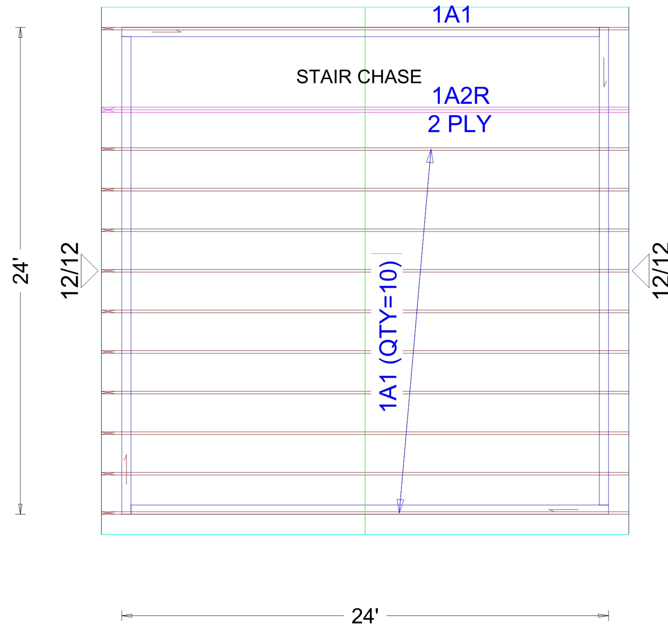
TRUSS LAYOUT
