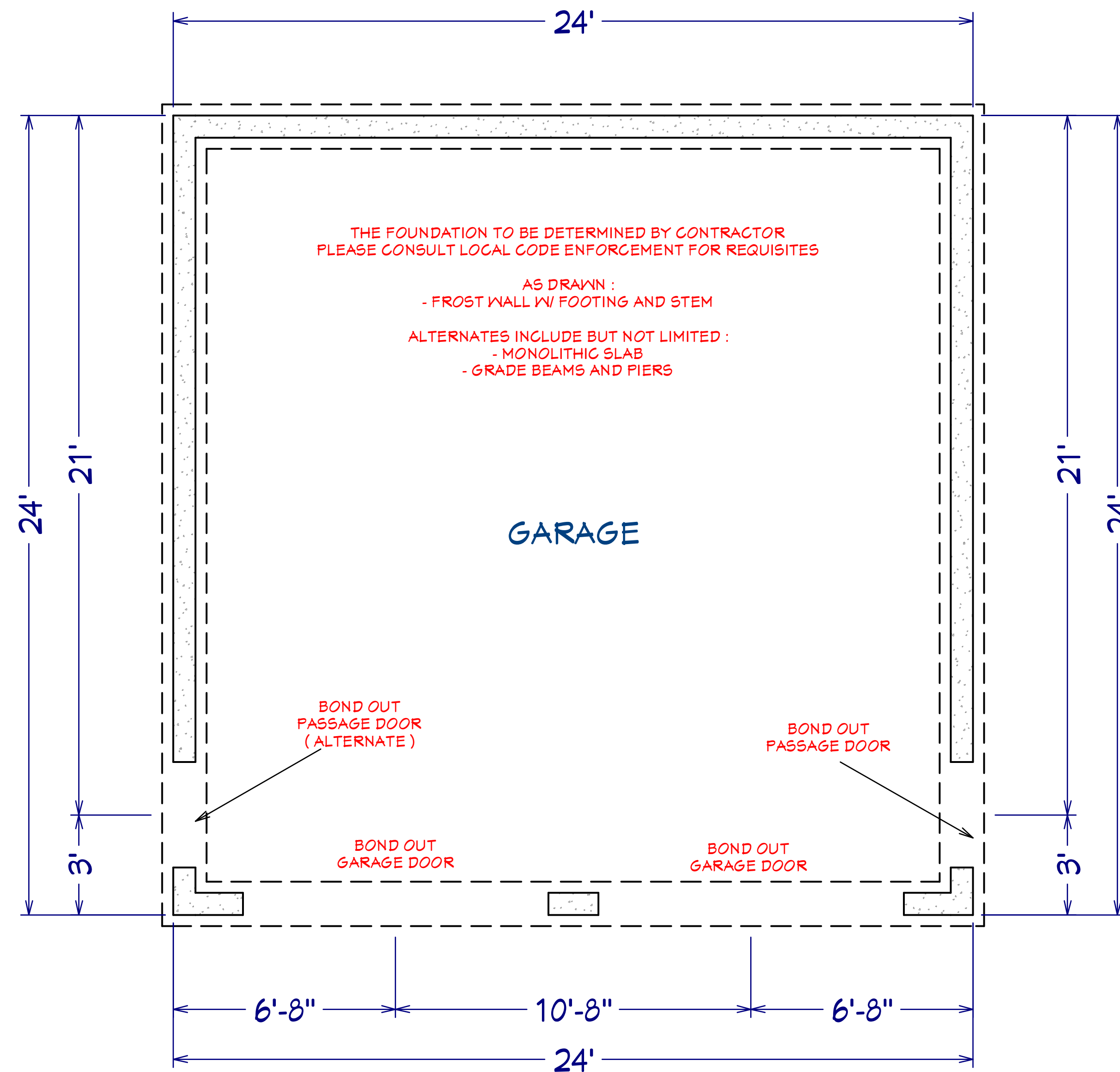
SLAB w/ FROST WALL
