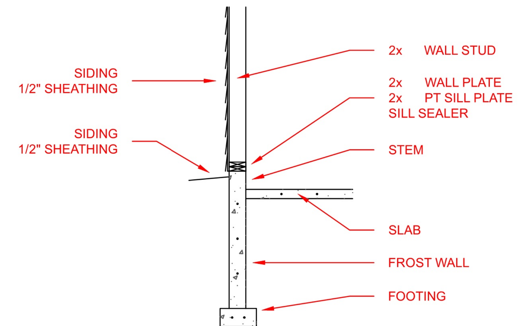
FOOTING w/ FROST WALL and STEM
